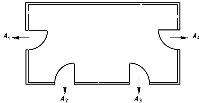
Figure A.1 — Leakage paths in parallel
