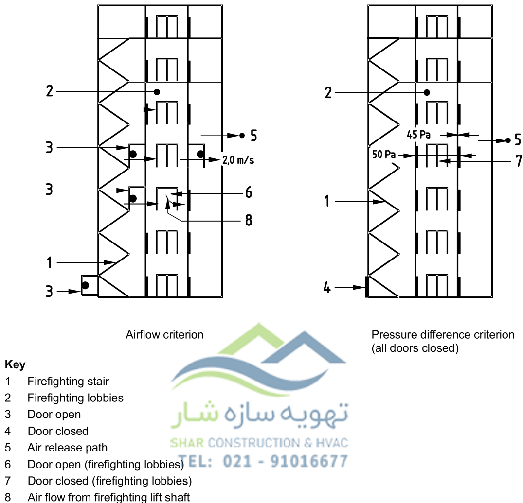
Figure 3 — Design conditions for Class B systems
