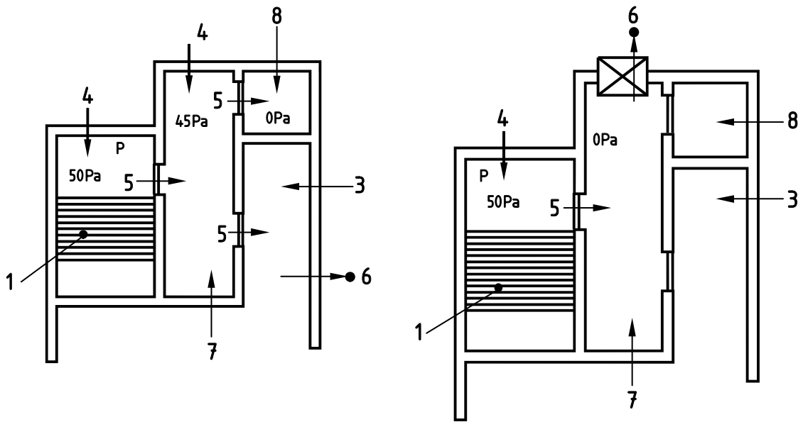
12 a) Pressurization to stairs and corridors
